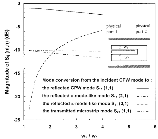
Fig. 4. Mode conversion of an incident CPW mode against asymmetry ratio of side-plane widths for w_1 + w_2 = 2.667 mm and f = 5 GHz. Other circuit dimensions are the same as those in Fig. 3.
